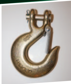
Grade 70 grab and slip hooks
